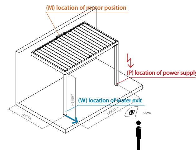
Type 2 - WALL-MOUNTED ON LENGTH SIDE
