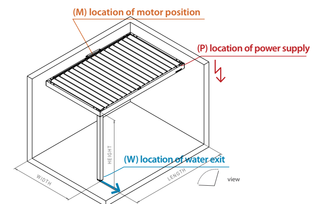
Type 3 - WALL-MOUNTED ON TWO SIDES
